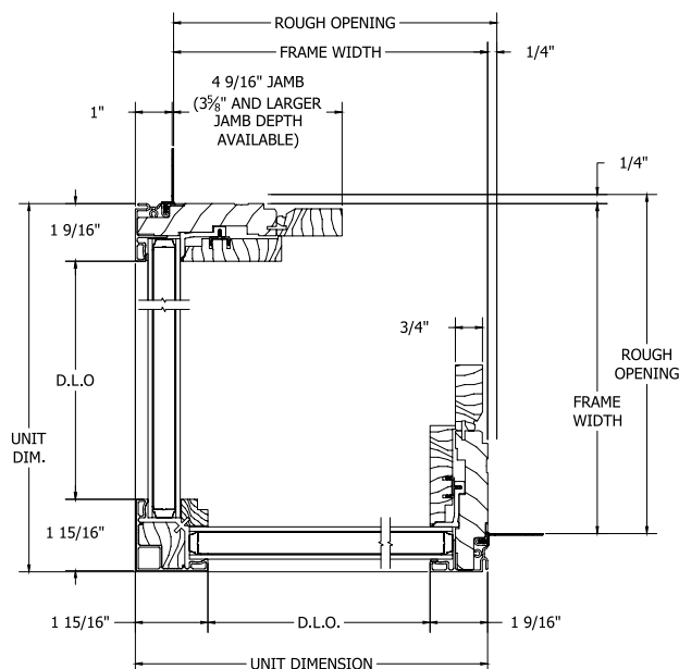
Horizontal Section
