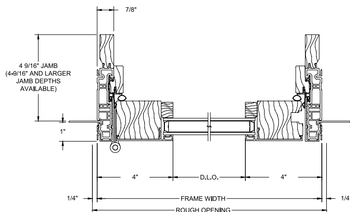
Horizontal Section
