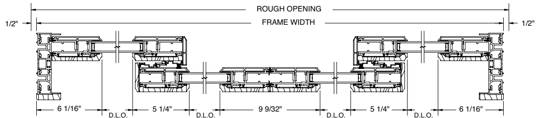
Horizontal Section
