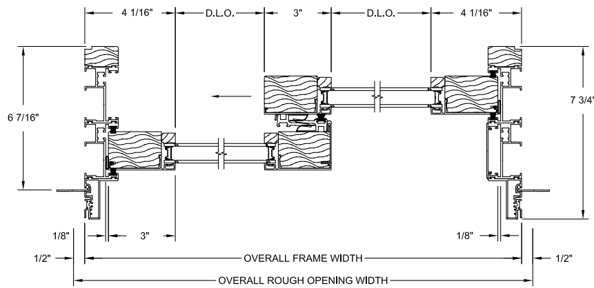
Horizontal Section
