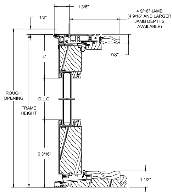
Vertical Section
