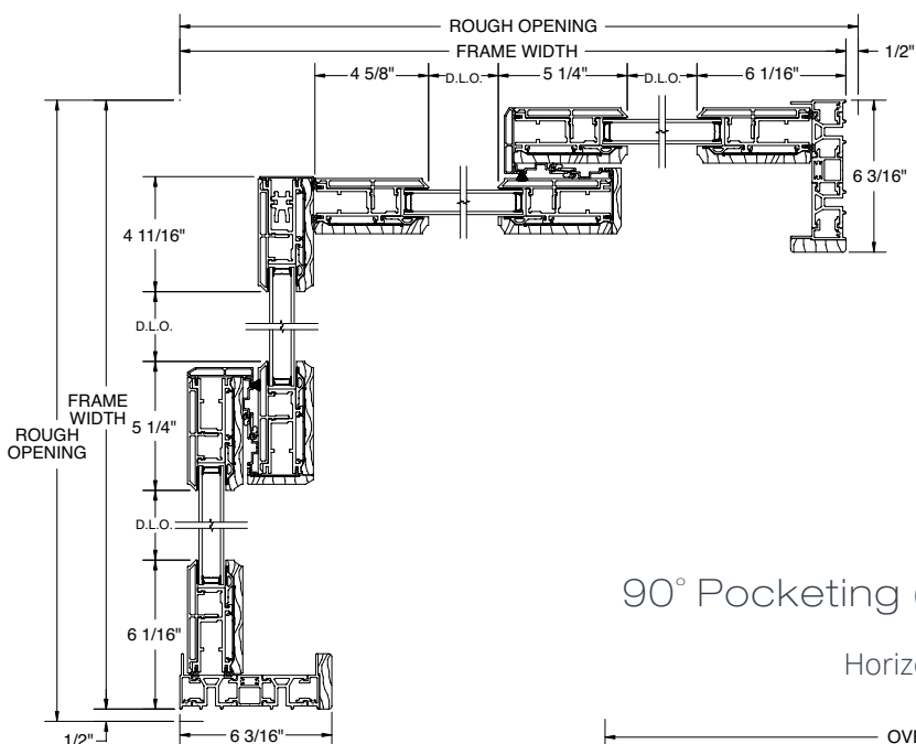
Horizontal Section
