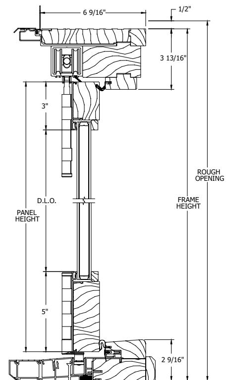
Vertical Section
