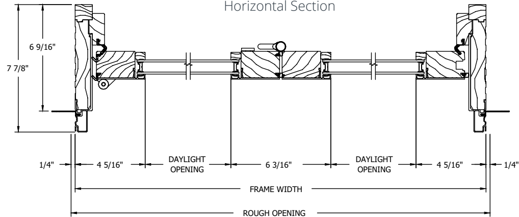
Horizontal Section
