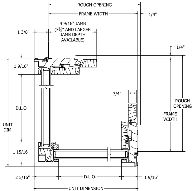
Horizontal Section
