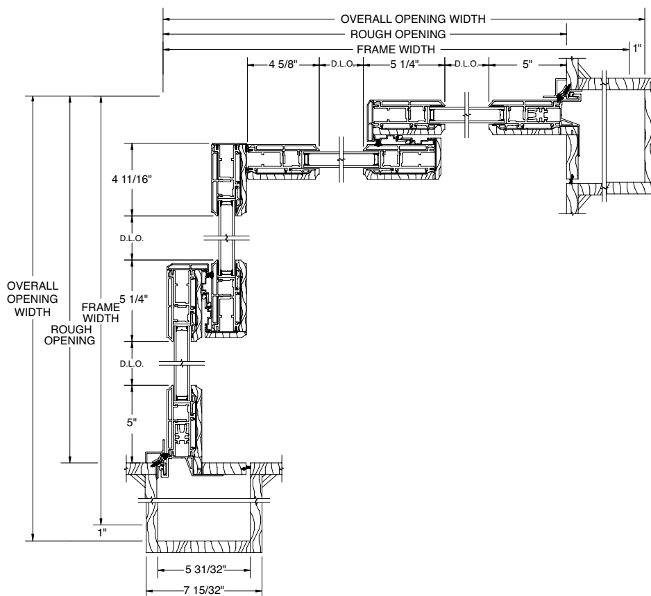
Horizontal Section
