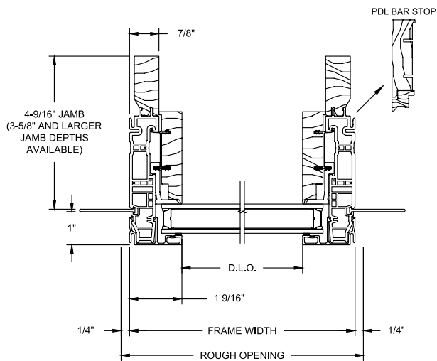
Horizontal Section
