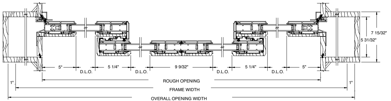
Horizontal Section
