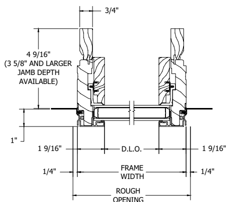
Horizontal Section
